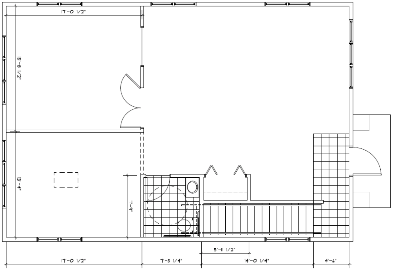
MAIN LEVEL PLAN
