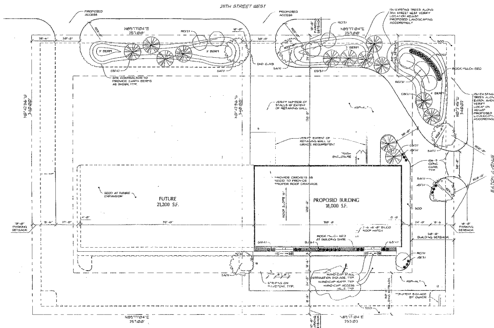
1 SITE & LANDSCAPING PLAN 1" = 30'
